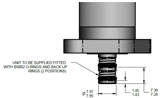
DETAIL A - SEALING O-RINGS
