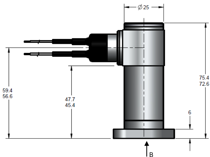
Flat Face Pressure Connection
