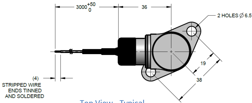
Top View - Typical
